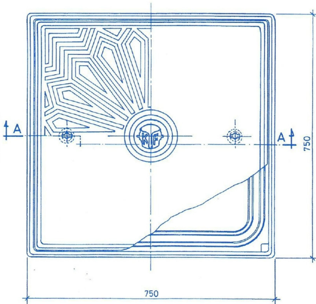
PLAN
