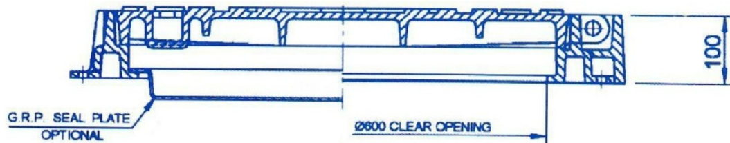
SECTION - AA
