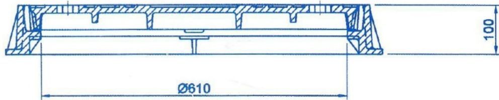
SECTION - AA
