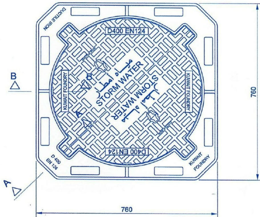
PLAN VIEW
