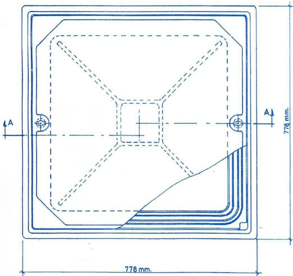
PLAN
