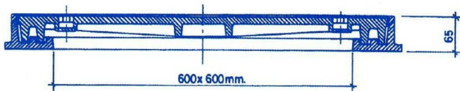
SECTION-AA
