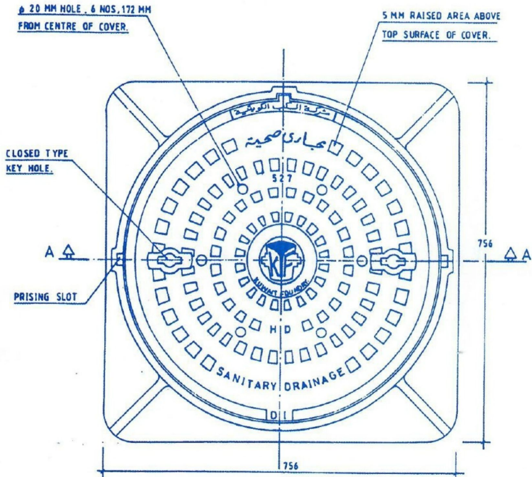
PLAN
