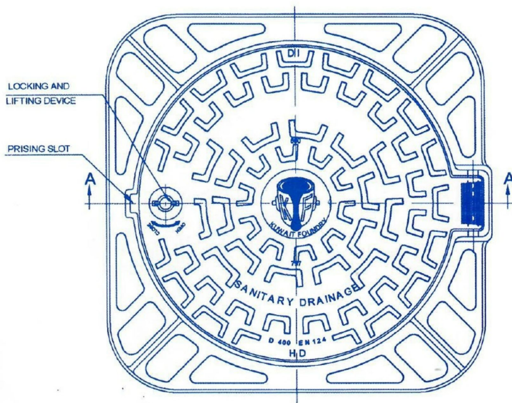
PLAN VIEW
