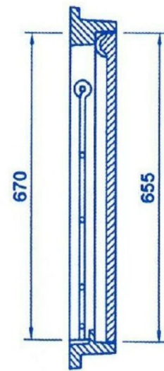
SECTION - BB
