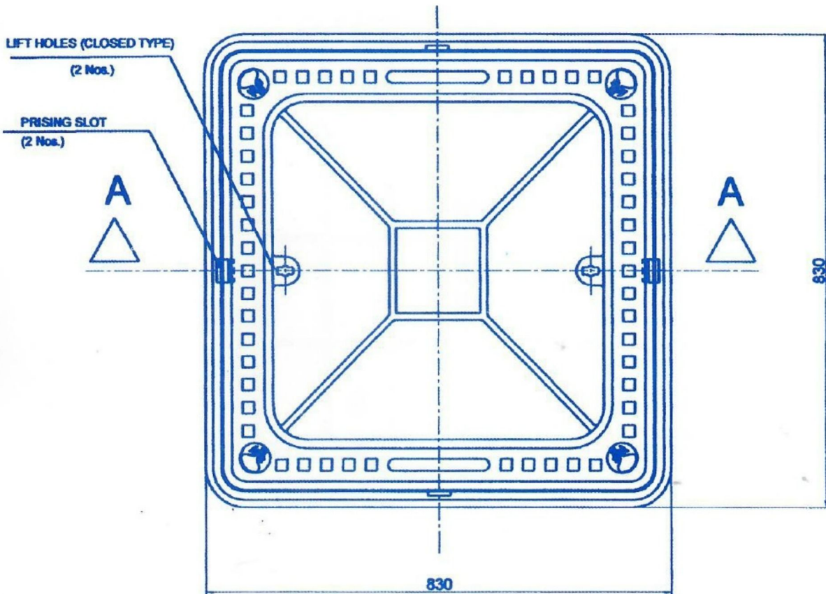
PLAN VIEW
