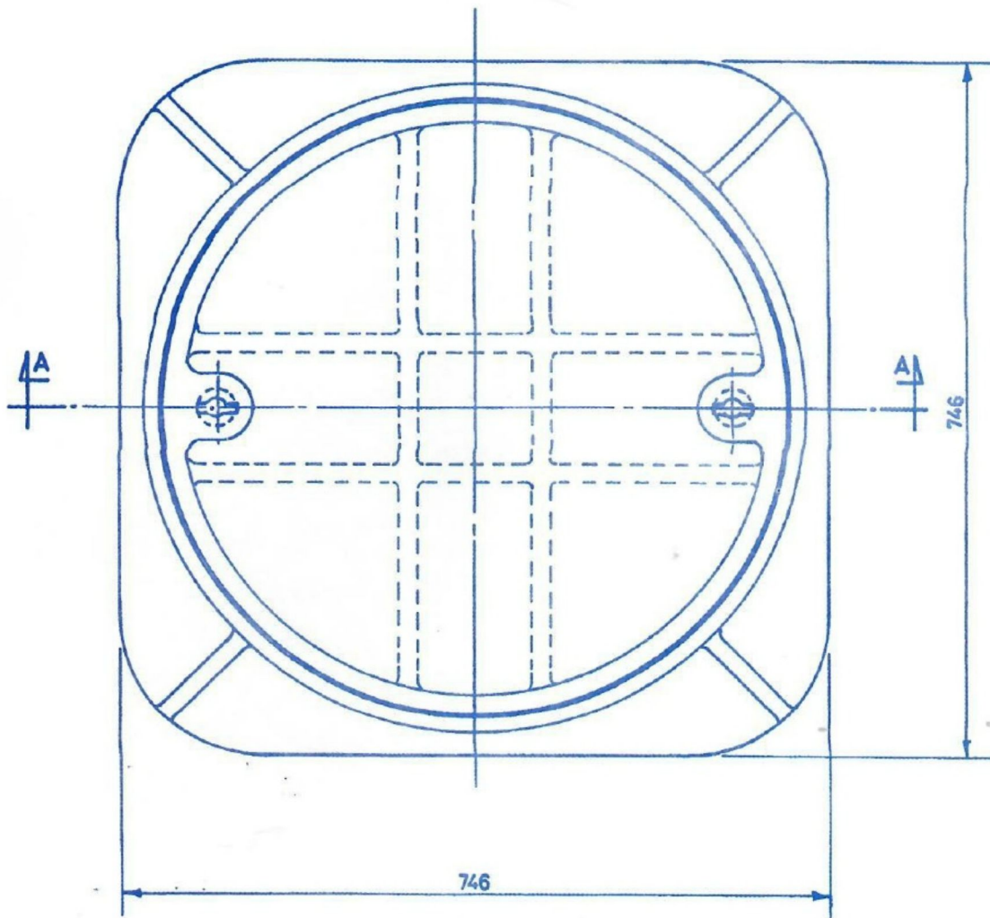
PLAN
